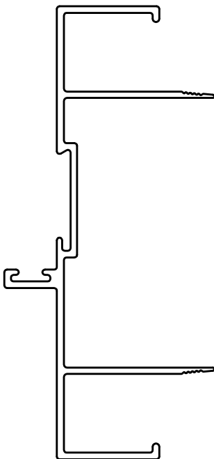
39397 GLAZING 1
