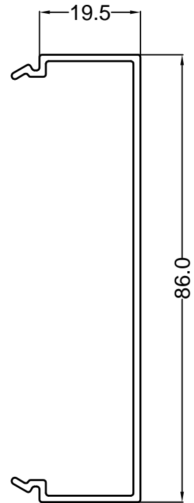
39382 TERMINATION 2
